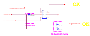
SP2T FOR B20_B28N71 ENDC PRX
